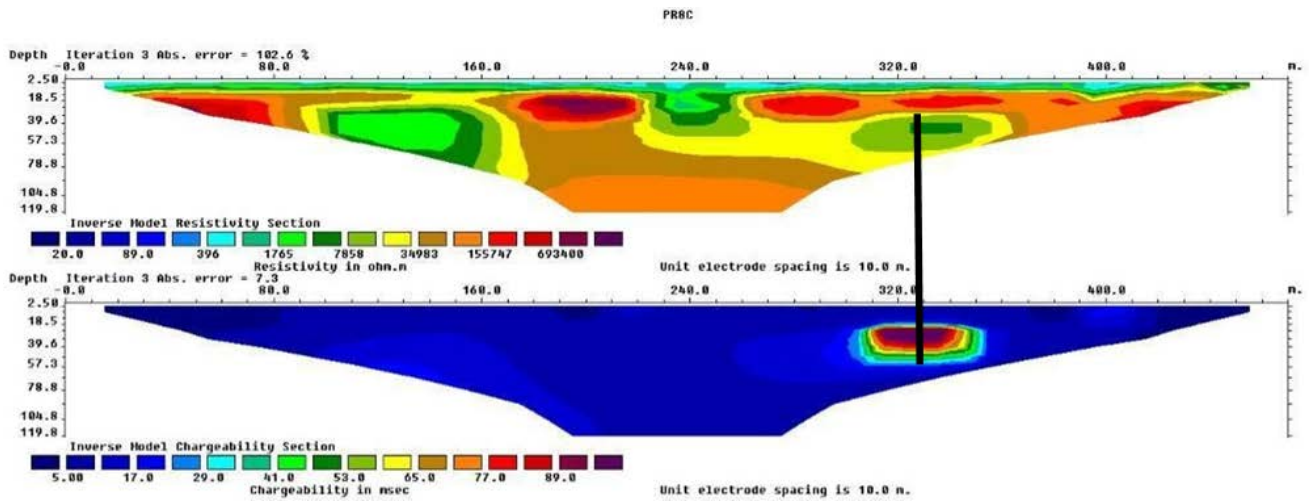
Figure 12. 2-D inverted IP-Resistivity mode plot for Profile 8C_East (290600 to 291070, 1050000)
