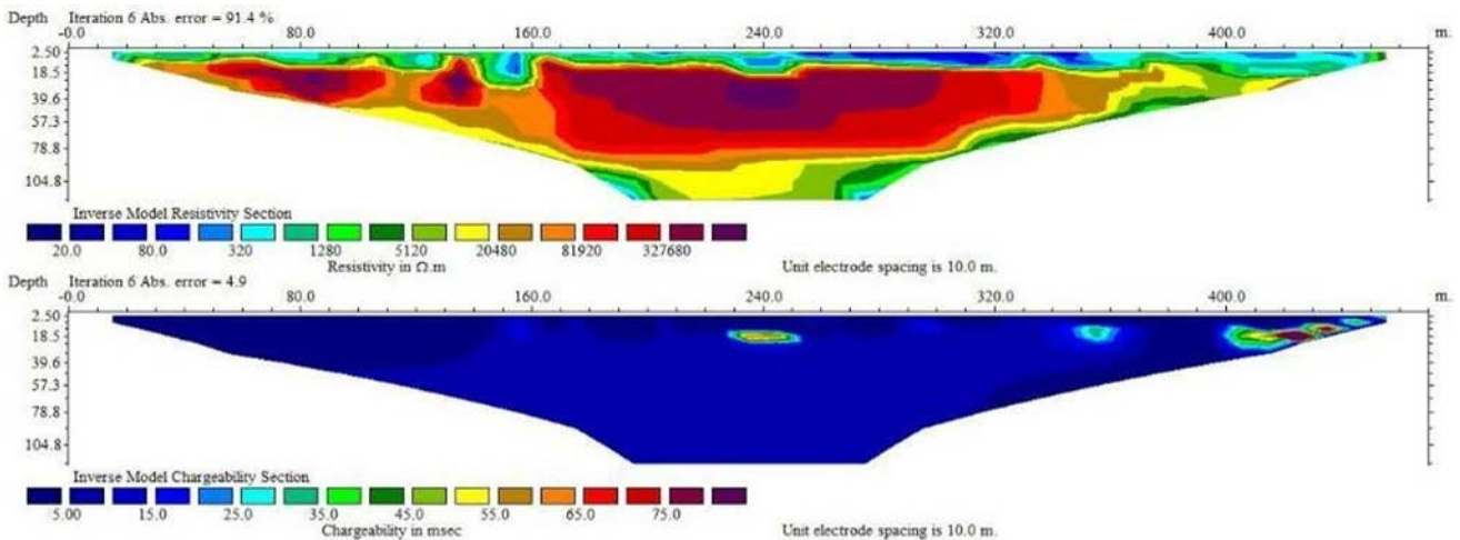
Figure 11. 2-D inverted IP-Resistivity mode plot for Profile 5C_West (290240 to 289773, 1050300)
