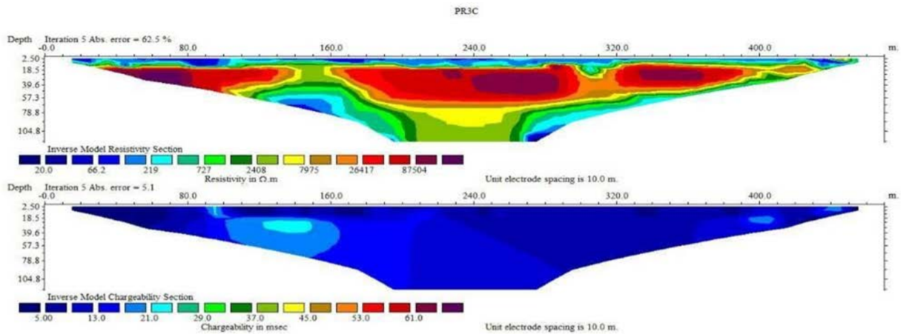
Figure 10. 2-D inverted IP-Resistivity mode plot for Profile 3C_West (290070 to 289597, 1050500)
