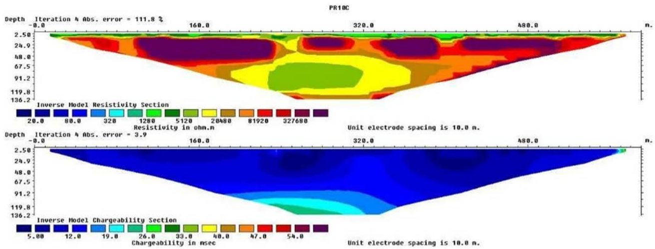
Figure 15. 2-D inverted IP-Resistivity mode plot for Profile 10C_West (290500 to 289907, 1049800)
