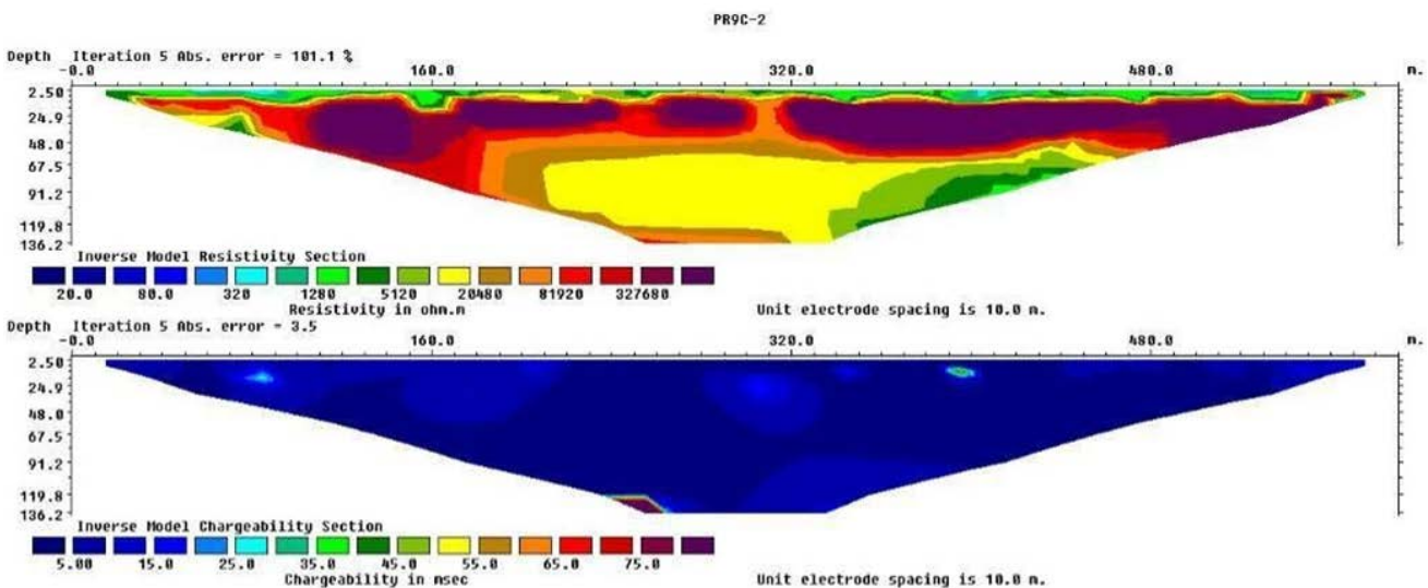
Figure 14. 2-D inverted IP-Resistivity mode plot for Profile 9C_West (290500 to 289908, 1049900)
