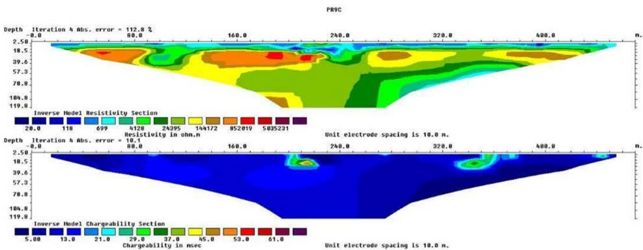
Figure 13. 2-D inverted IP-Resistivity mode plot for Profile 9C_East (290600 to 291069, 1049900)
