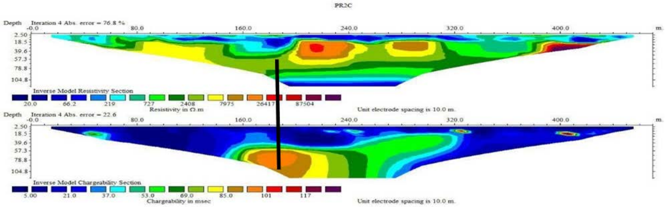
Figure 9. 2-D inverted IP-Resistivity mode plot for Profile 2C_West (290045 to 289571, 1050600)
